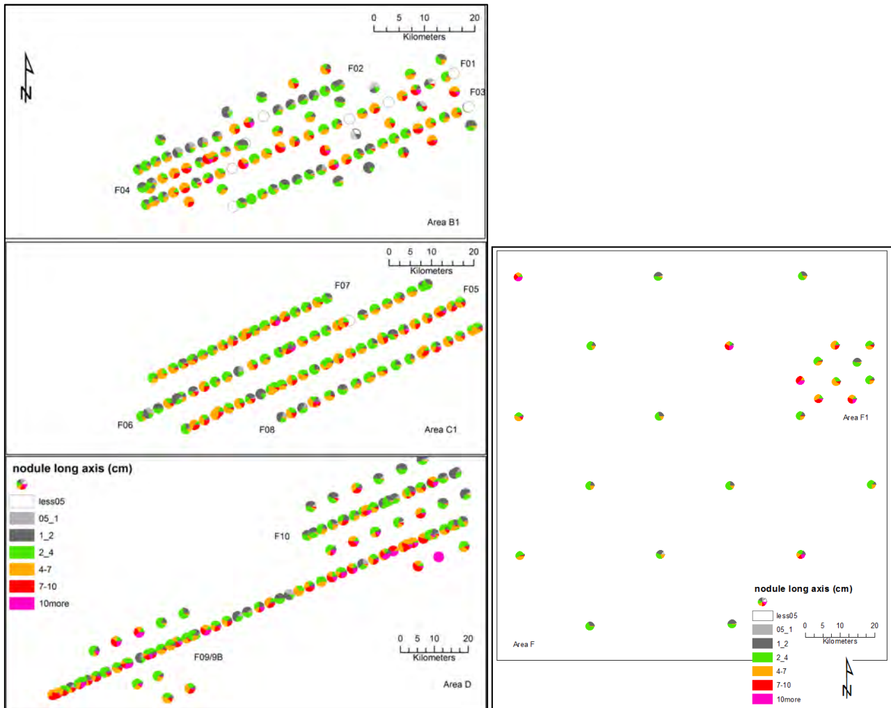
Figure 7.53 Nodule sizes and types from photo-profiles and box-cores
