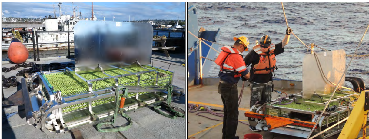
Figure 7.30 Photos of epibenthic sled
