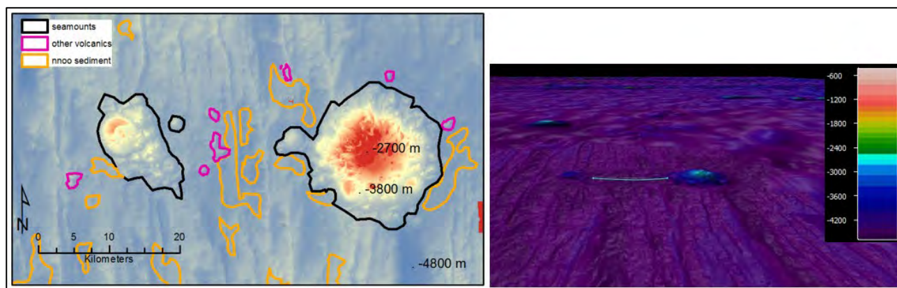
Figure 6.4 Seamounts in TOML Area D
