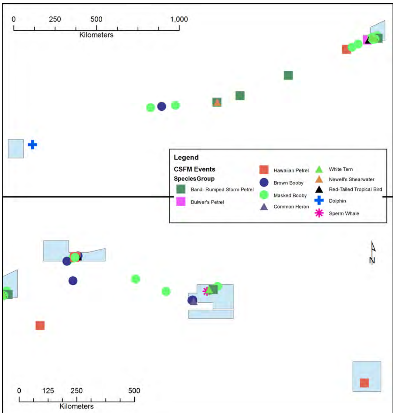
Figure 7.34 CCZ15 CSMF Events
