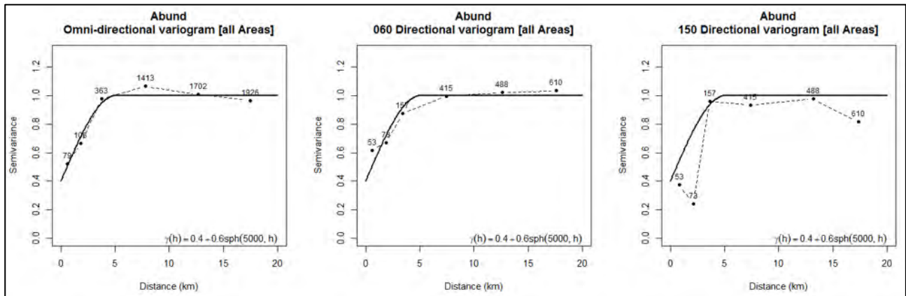
Figure 11.25 Abund omni-directional, 060° and 150° directional variograms
