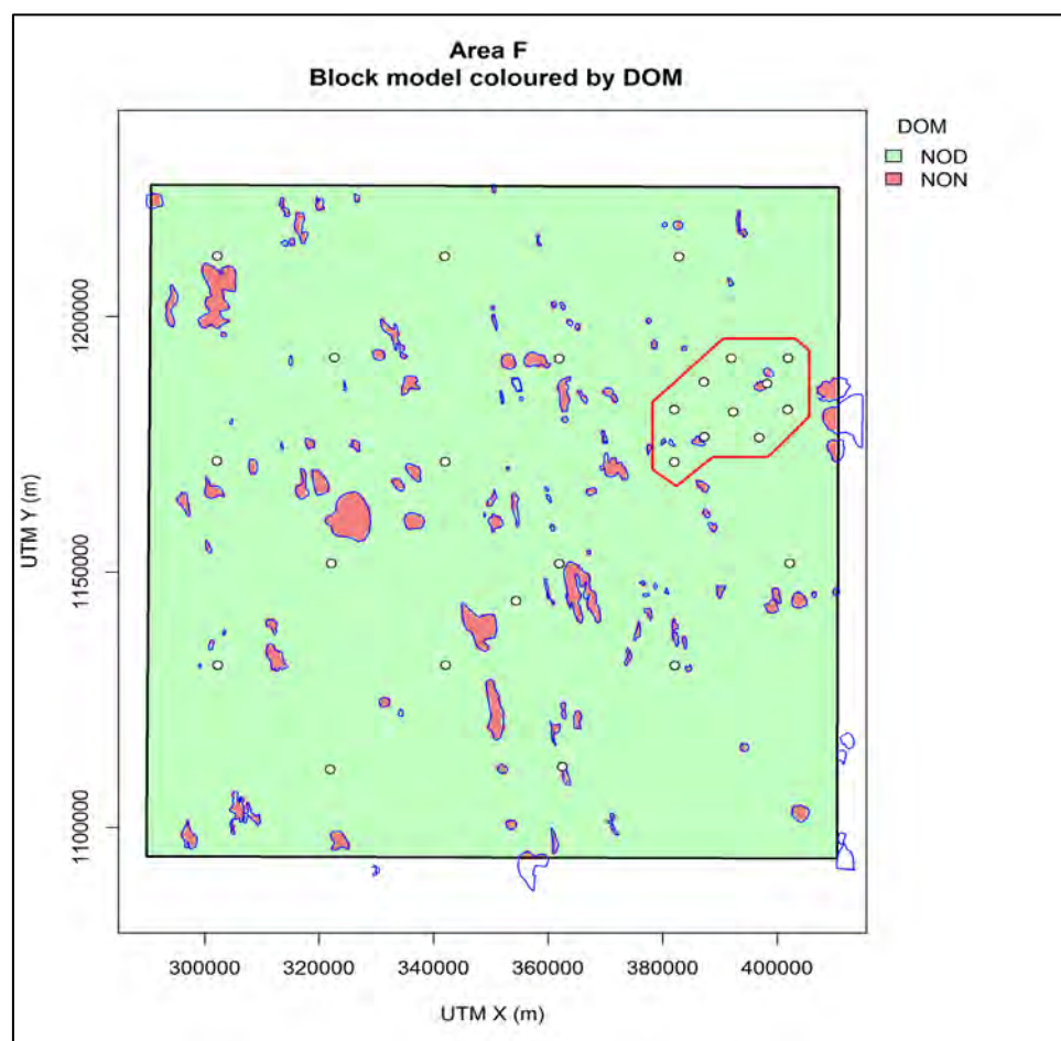
Figure 11.5 TOML Exploration Area F geological domains
