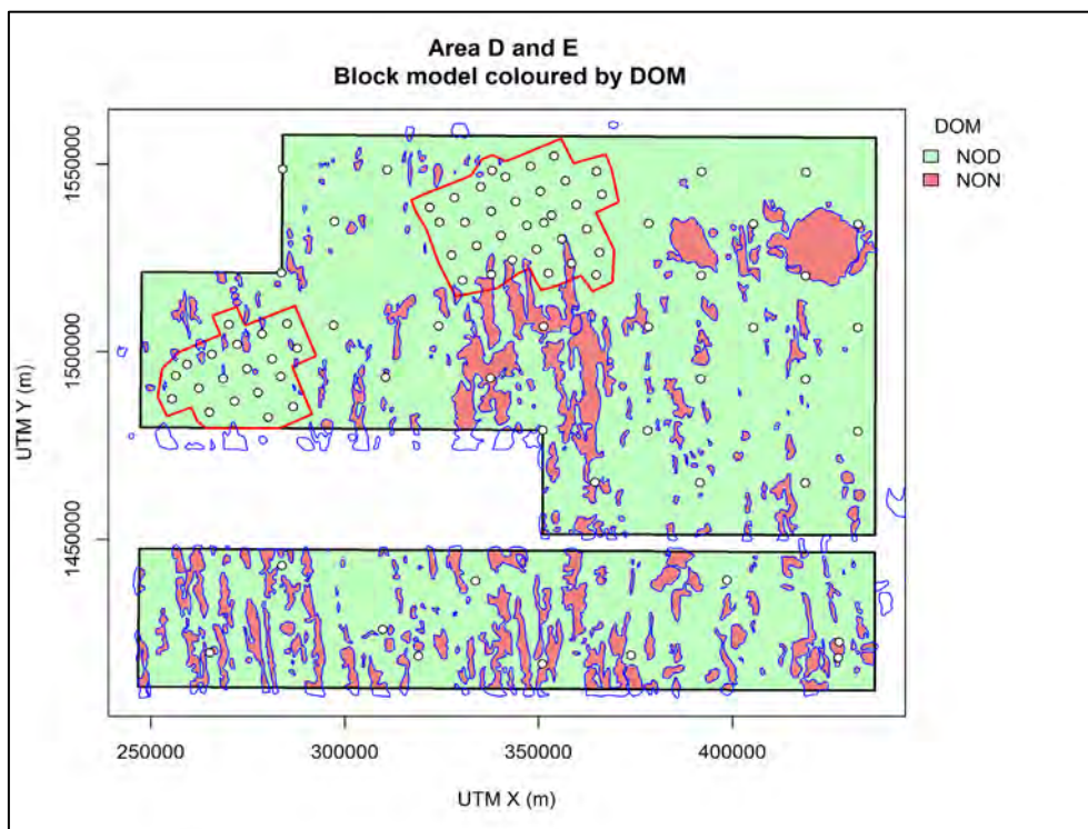
Figure 11.4 TOML Exploration Area D and E geological domains
