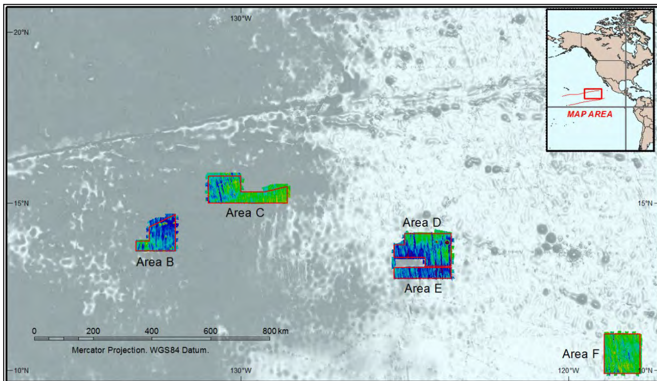
Figure 7.35 CCZ13 MBES bathymetry coverage
