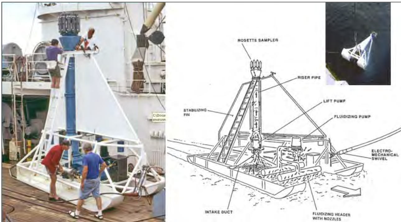
Figure 5.19 DSSRS-II Benthic Disturber
