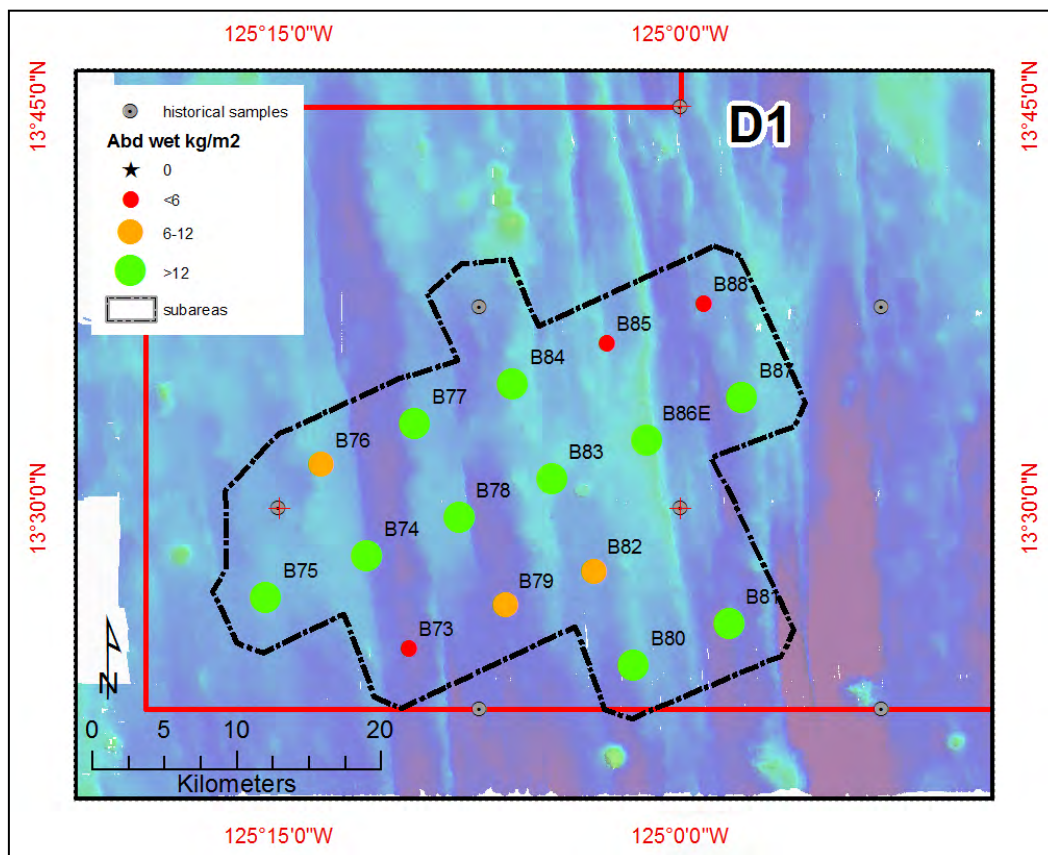
Figure 7.47 Nodule Abundance, Area D1
