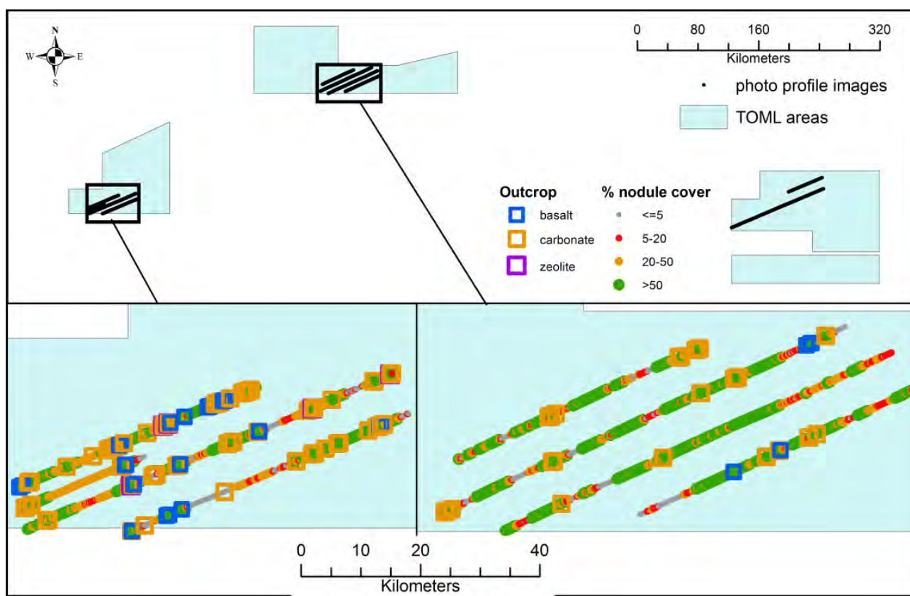
Figure 7.52 Neptune Photo-profile logging of % cover and outcrop types
