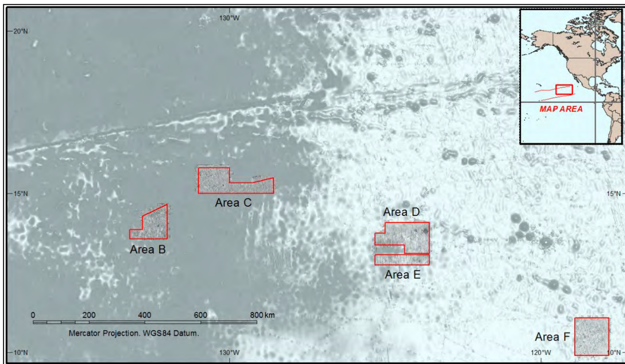
Figure 7.36 CCZ13 MBES backscatter coverage
