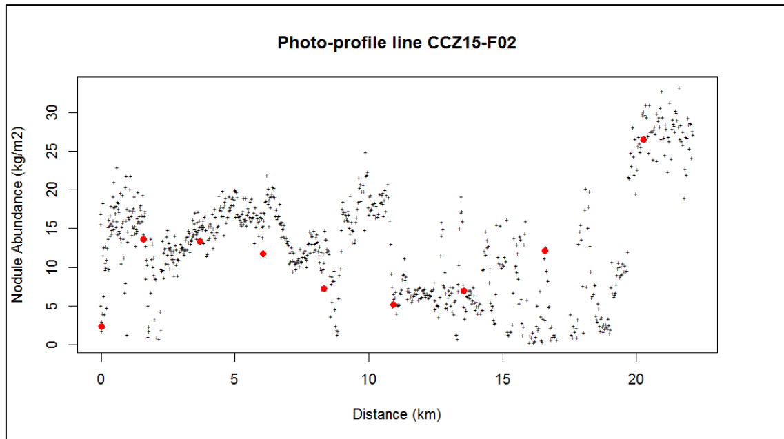
Figure 11.23 Nodule abundance photo-profile line CCZ15-F02 that crosses sub-area B1 Measured Mineral Resource
