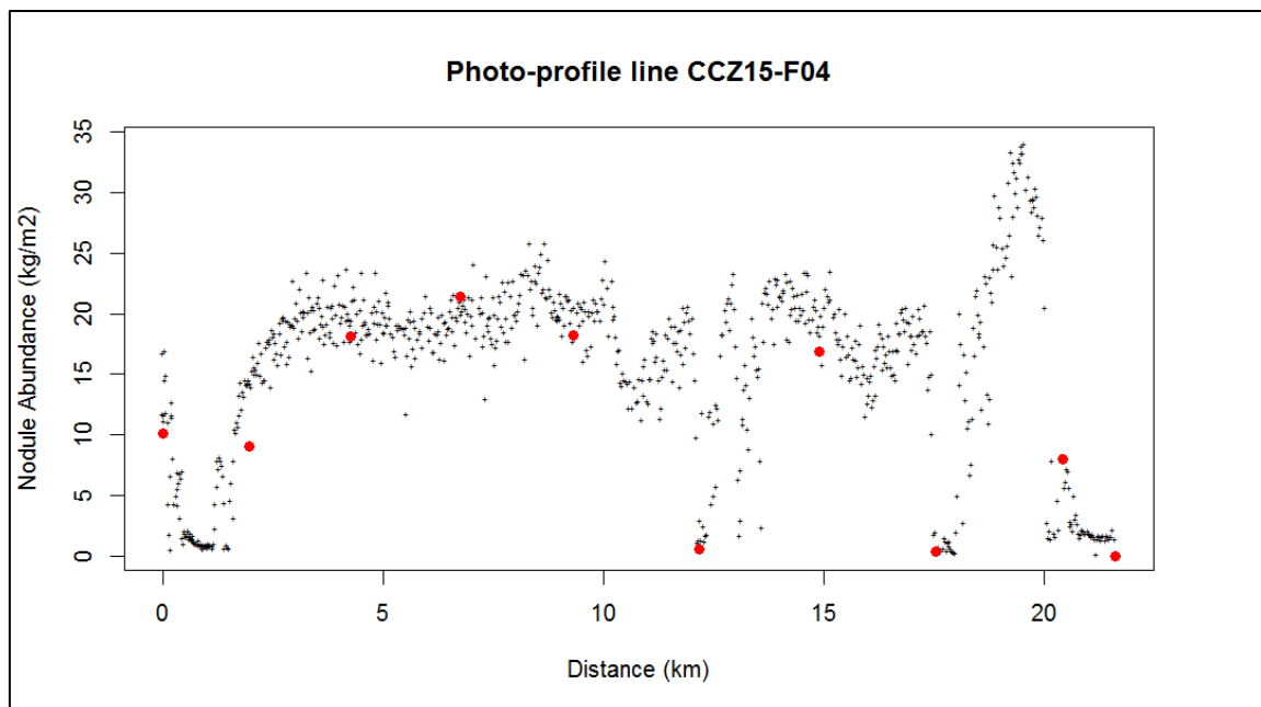
Figure 11.24 Nodule abundance photo-profile line CCZ15-F04 that crosses sub-area B1 Measured Mineral Resource
